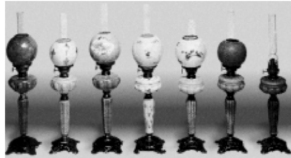
Abb. 2002-2/039 Gepresste Feuerstein-Lampen Fostoria Shade and Lamp Co., Fostoria, Ohio, 1890 ab 1894 Consolidated Lamp & Glass Co.
